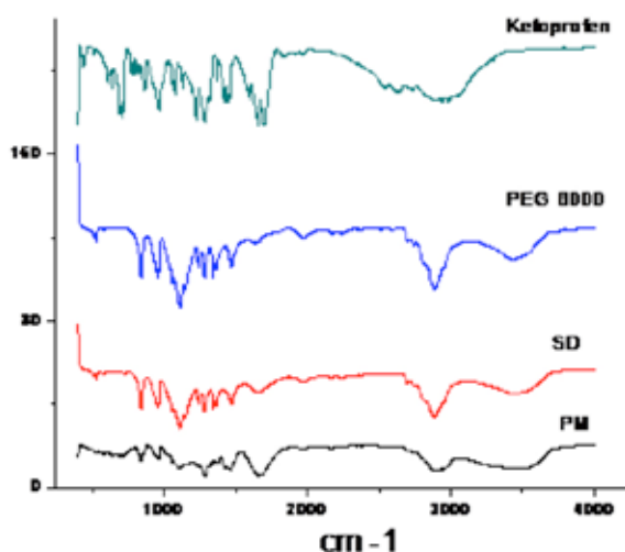
Figure 1. FTIR spectra of pure ketoprofen, PEG 6000, SD and physical mixture.
